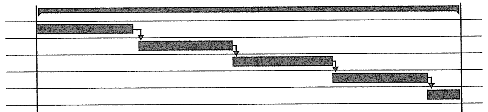
Model 2 – Waterfall
