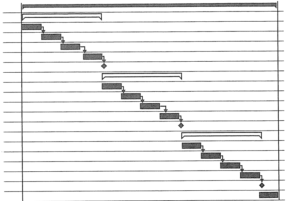
Model 1 – Agile
